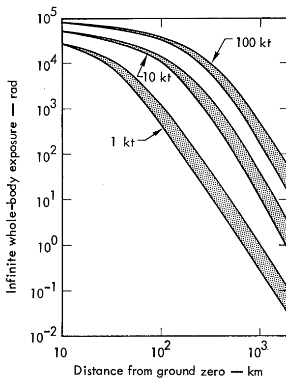
Fig. 16. Vertical integral (infinite whole-body exposure) due to gross \gamma radiation as a function of distance from ground zero. The upper curve for each yield represents the case of slow horizontal diffusion; the lower curve represents the case of fast diffusion. (From Ref. 33.)
